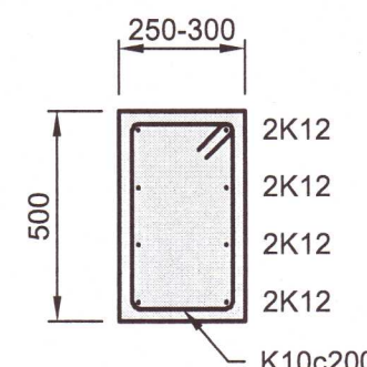
17 SNID 1:20
