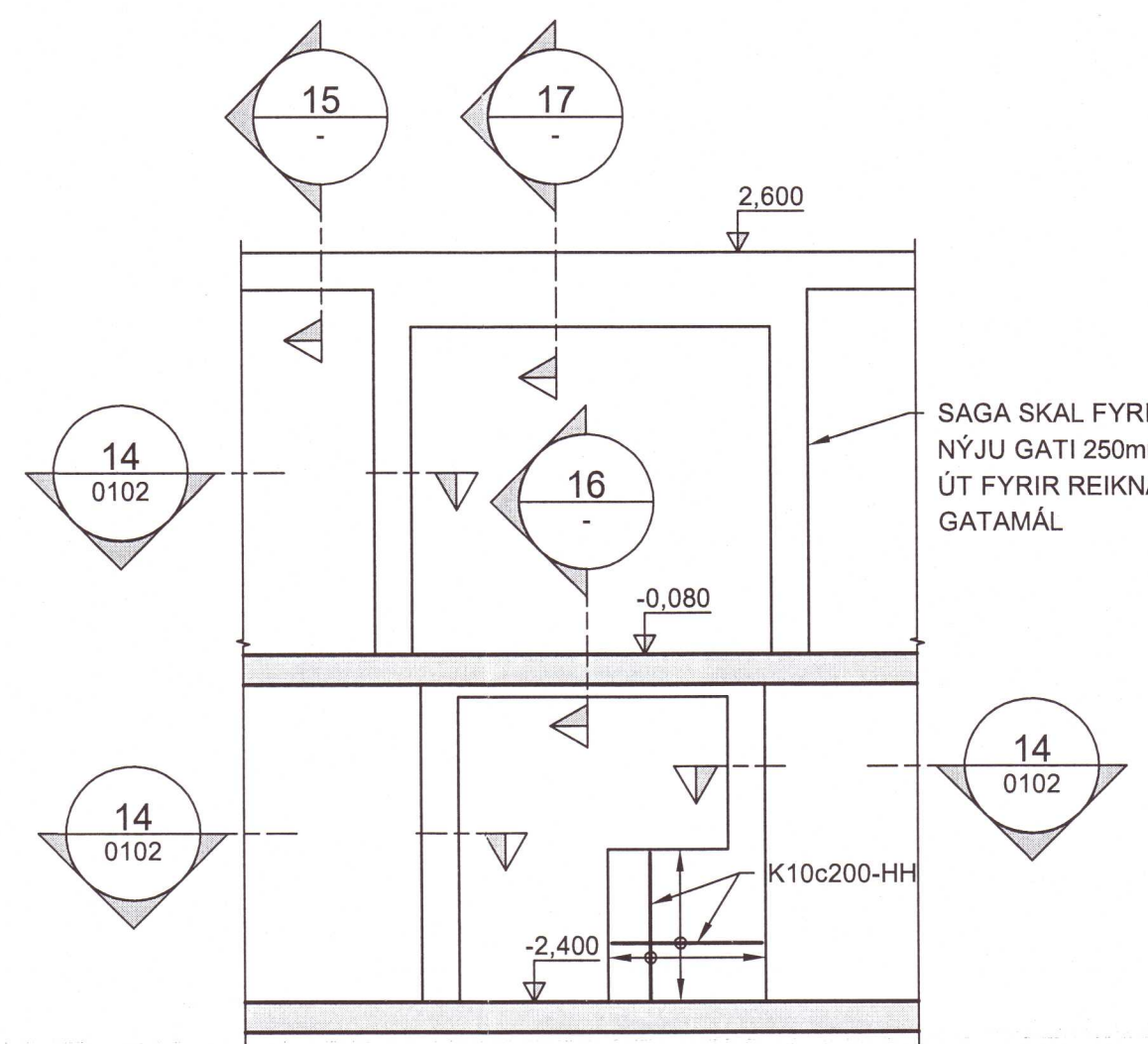
18 SNID 1:50
