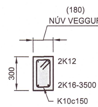
20 SNID 1:20
