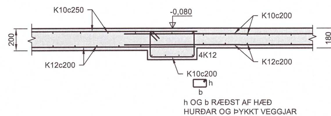
16 SNID 1:20
