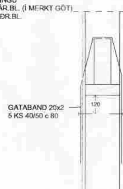
SNID C-C
