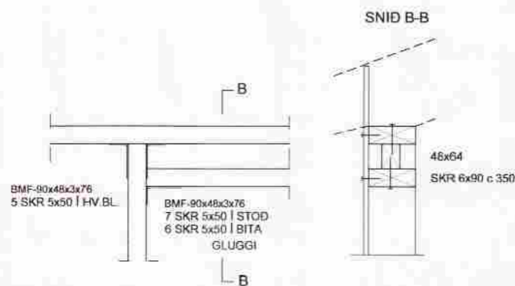
SNID 28 1:10
