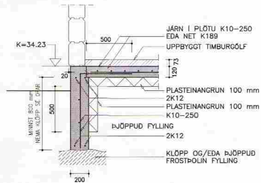
SNID 3-3 1:20
