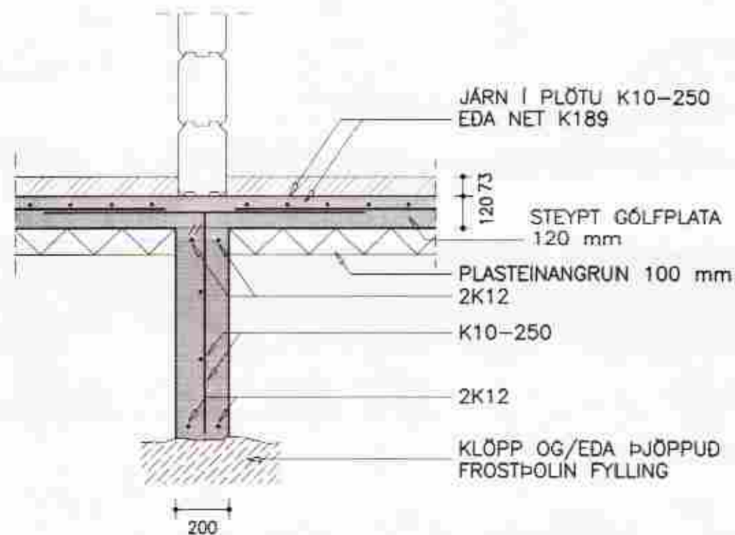
SNID 4-4 1:20
