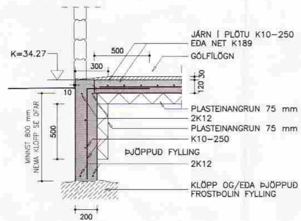
SNID 2-2 1:20
