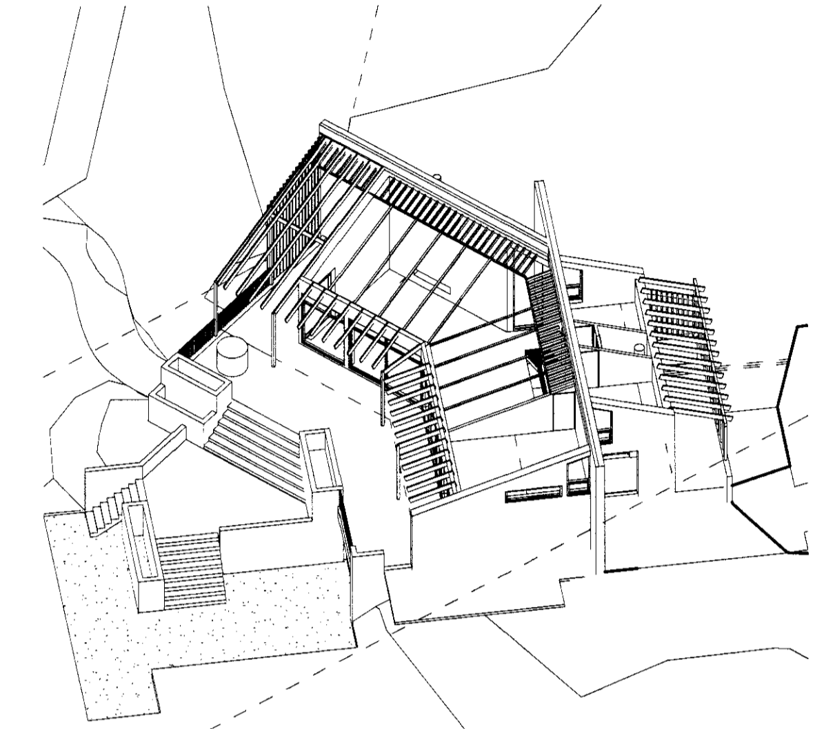
3d burðargrind
