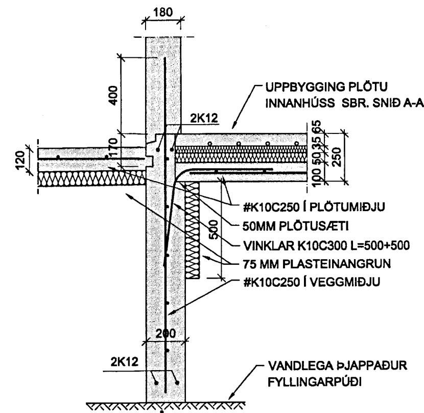
F SNEIÐING 01 Mkv. 1/20
