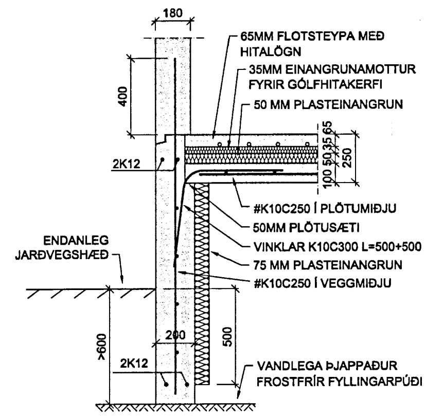
A SNEIÐING 01 Mkv. 1/20
