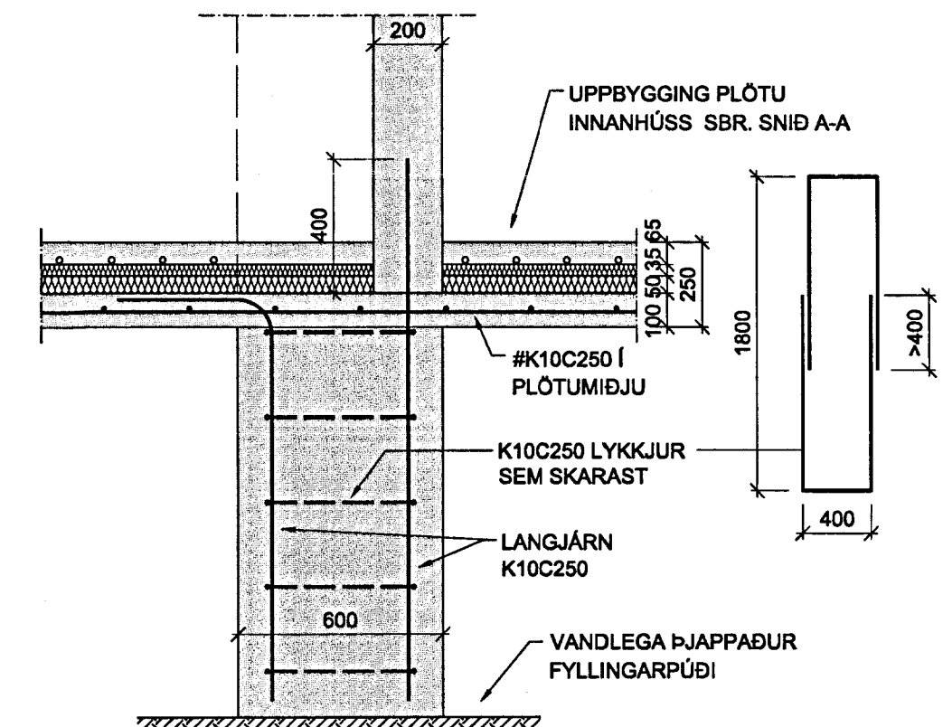
H SNEIÐING 01 Mkv. 1/20
