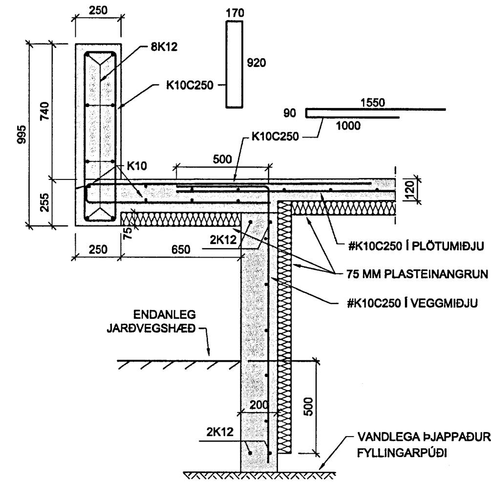
C SNEIÐING 01 Mkv. 1/20
