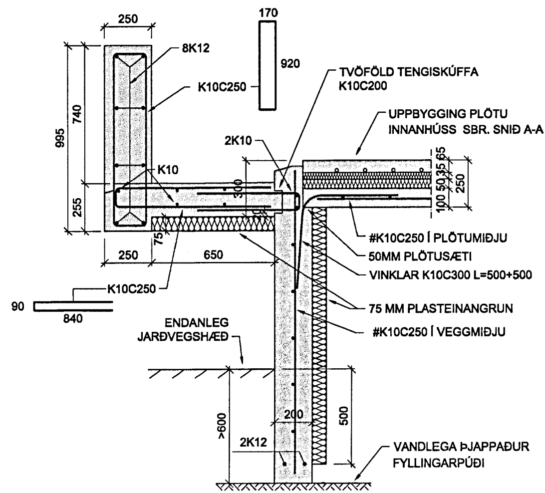
B SNEIÐING 01 Mkv. 1/20
