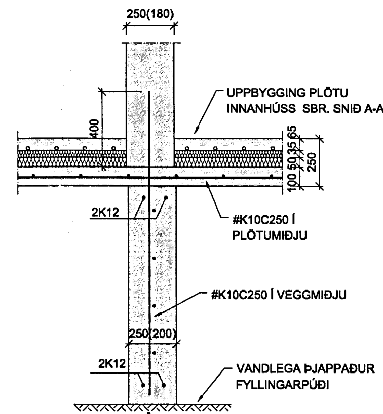
G SNEIÐING 01 Mkv. 1/20
