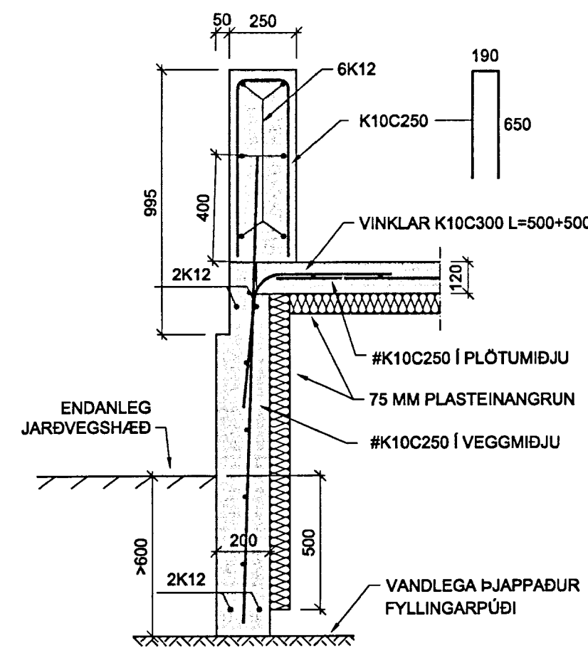
D SNEIÐING 01 Mkv. 1/20
