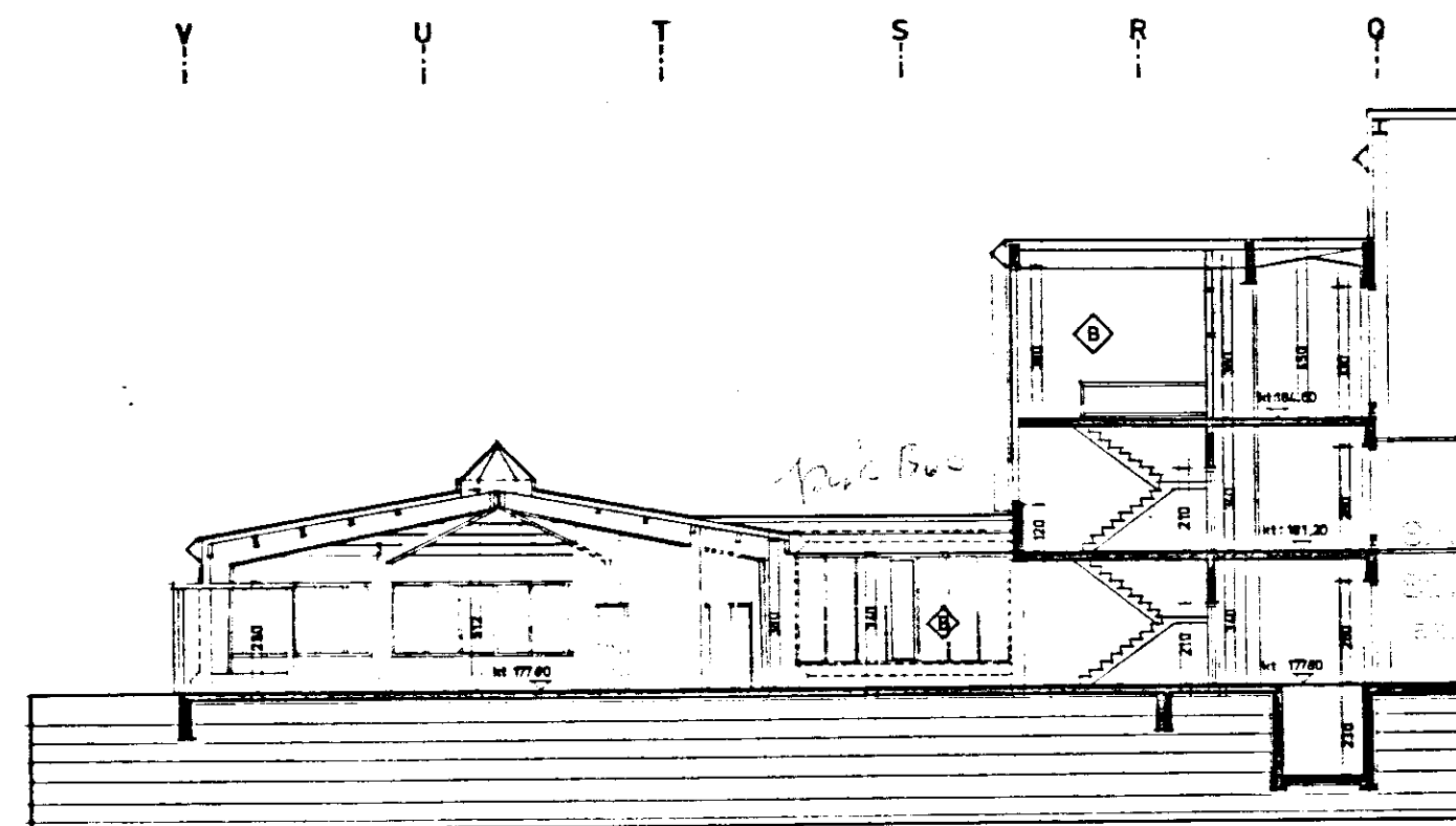
sneiding H-H
