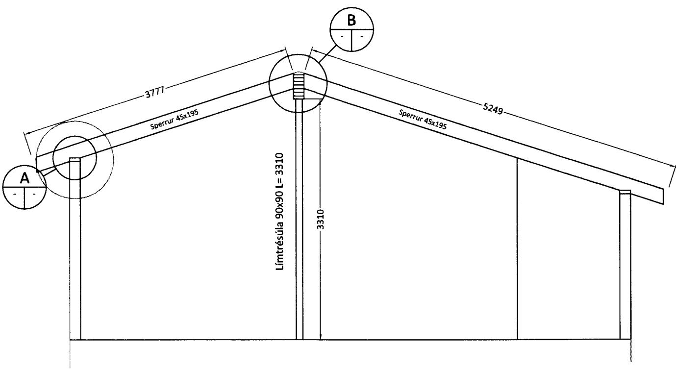
SNID A 1:50
