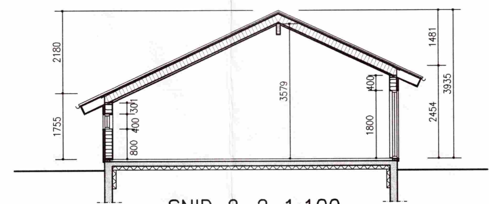
SNID 2-2 1:100
