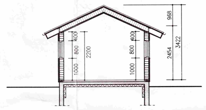
SNID 3-3 1:100
