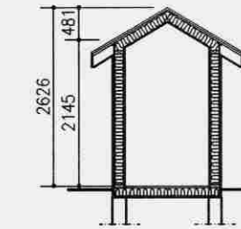
SNID 3-3 1:100
