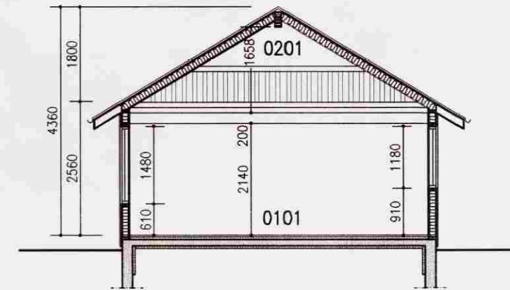
SNID 2-2 1:100
