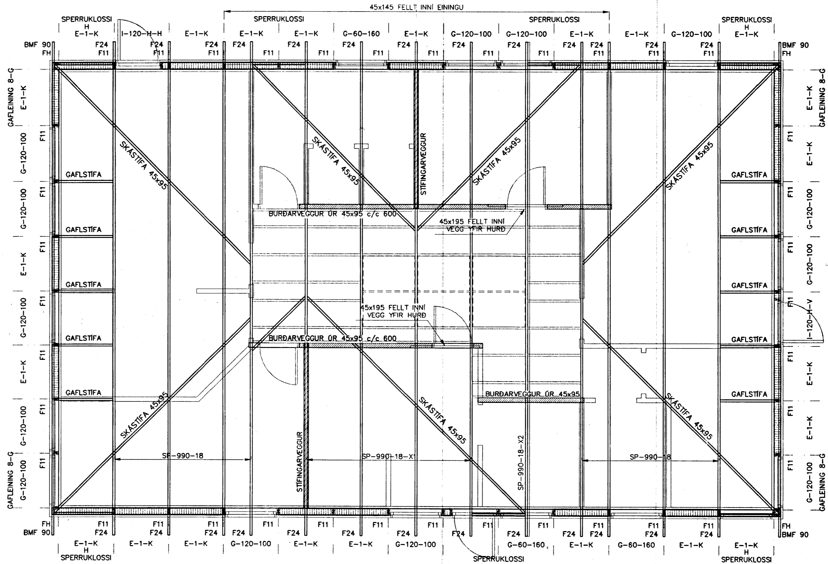
ÞAKPLAN Mkv. 1:50
