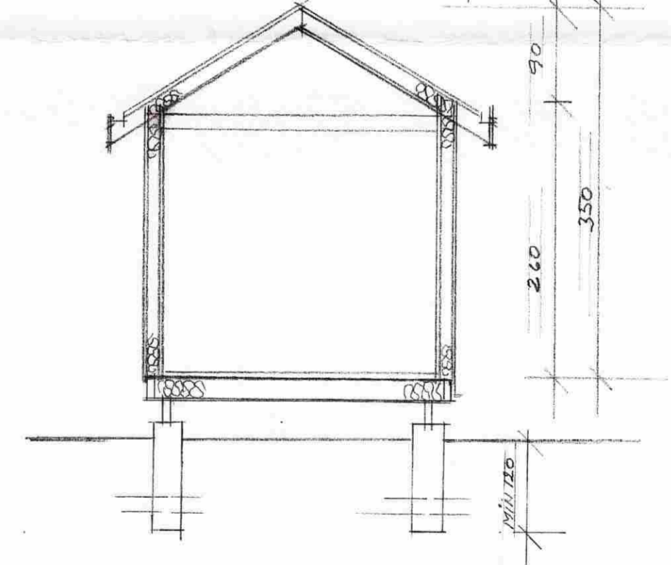
SNID C-C M=1:50
