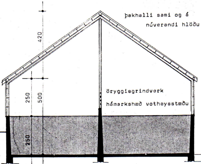
SNID A - A
