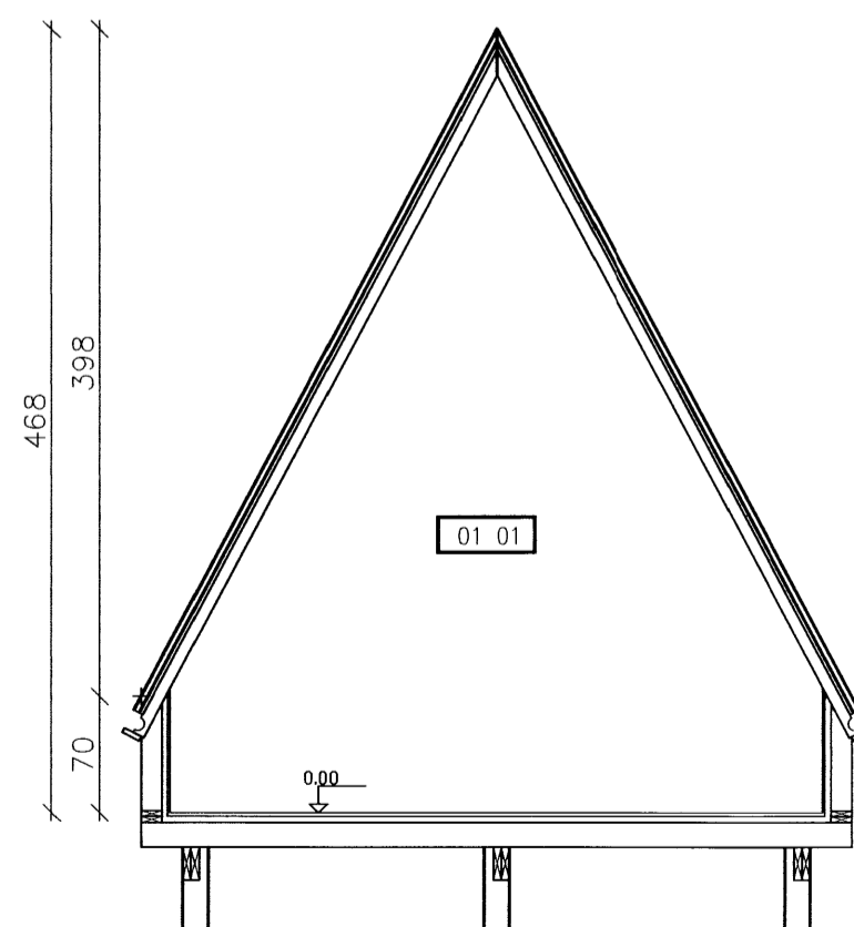
SNID B-B
