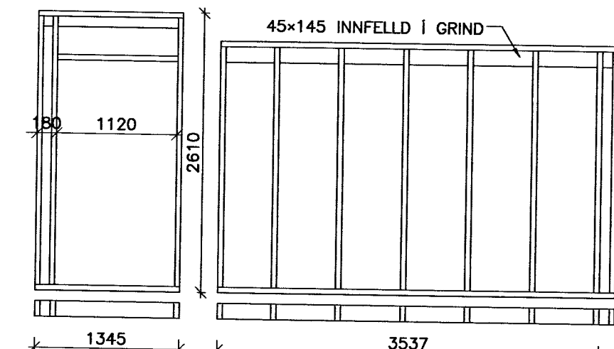
VEGGUR (11) 1:50
