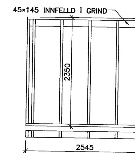
VEGGUR (8) 1:50
