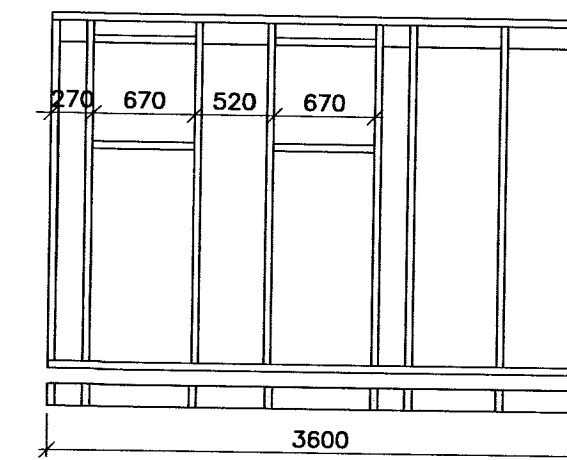
VEGGUR (9) 1:50
