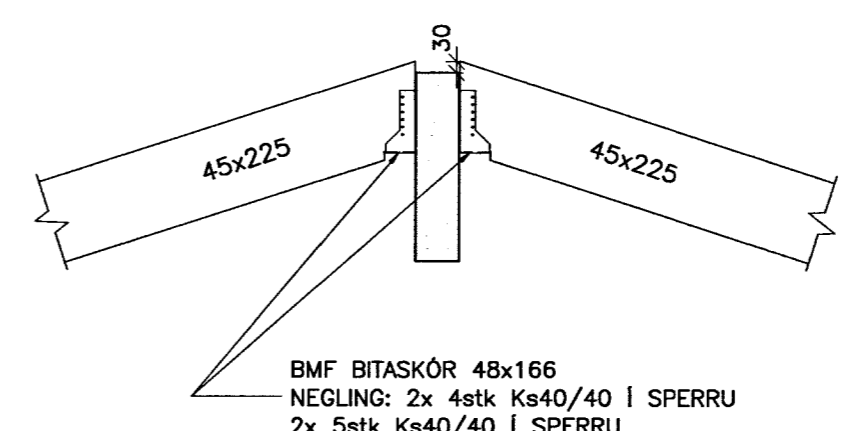
SNID B 1:20
