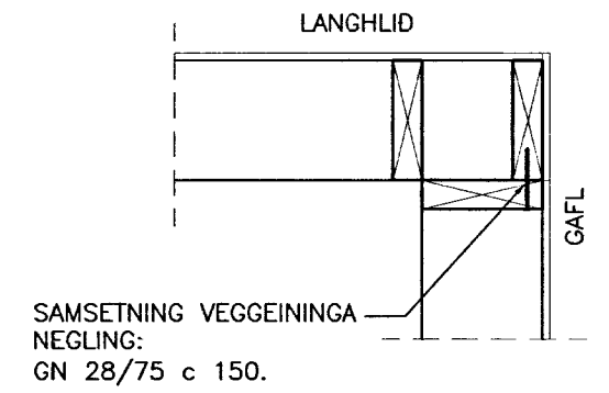
SNID D 1:10
