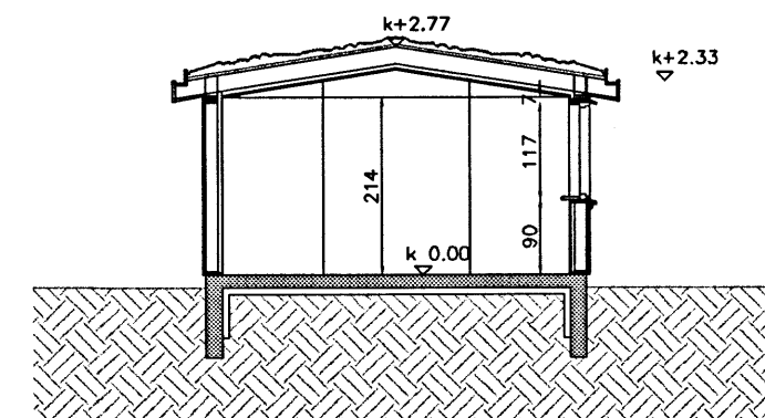
SNEIDING C-C MATSHLUTI 02
