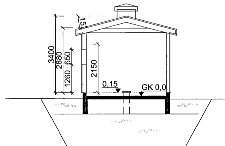
SNID 1:100
