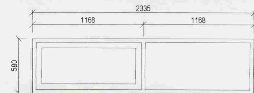
G-09, 1.stk M= 1:25
