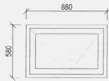
G-01, 1.stk M= 1:25
