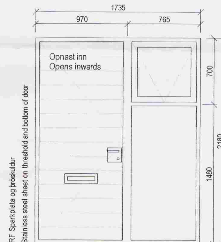
H-01, 1.stk M= 1:25
