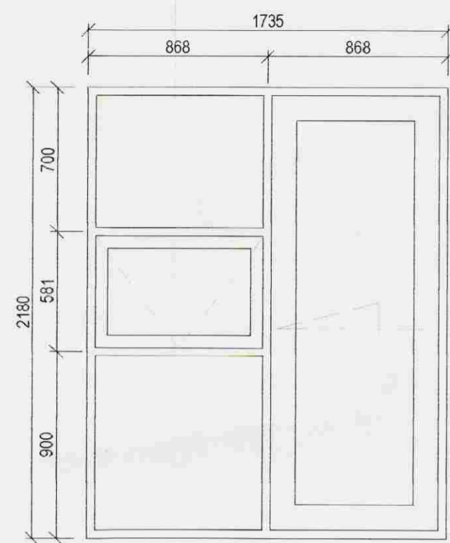
G-03, 1.stk M= 1:25
