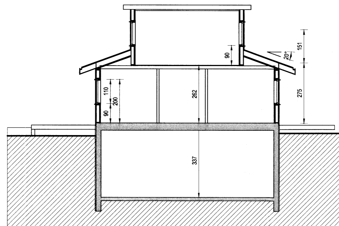
SNID B-B
