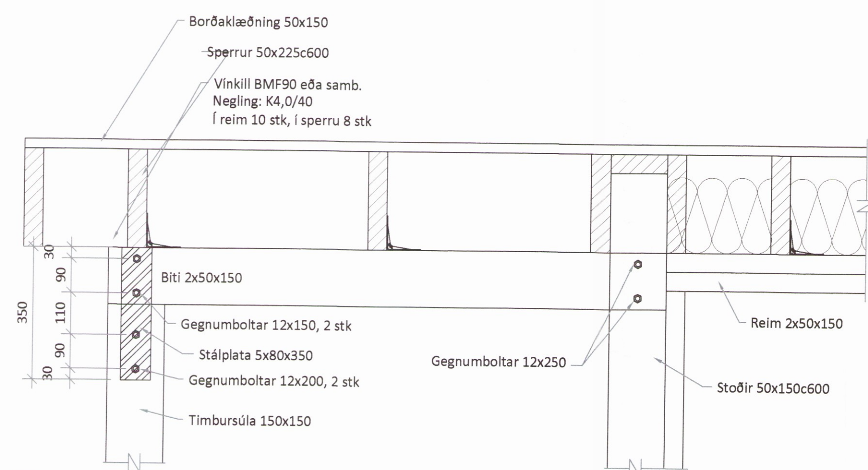
8 SNID 101 | 102 Mkv. 1:10
