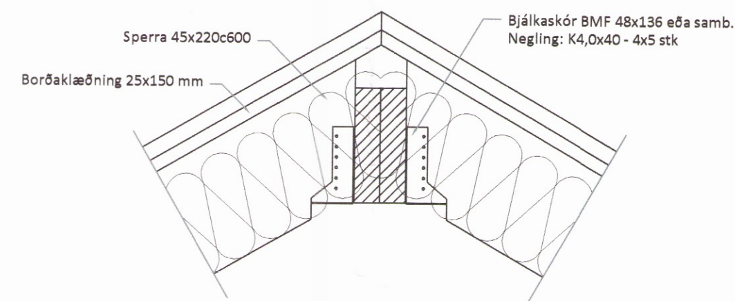
4 SNID 101 | 102 Mkv. 1:10
