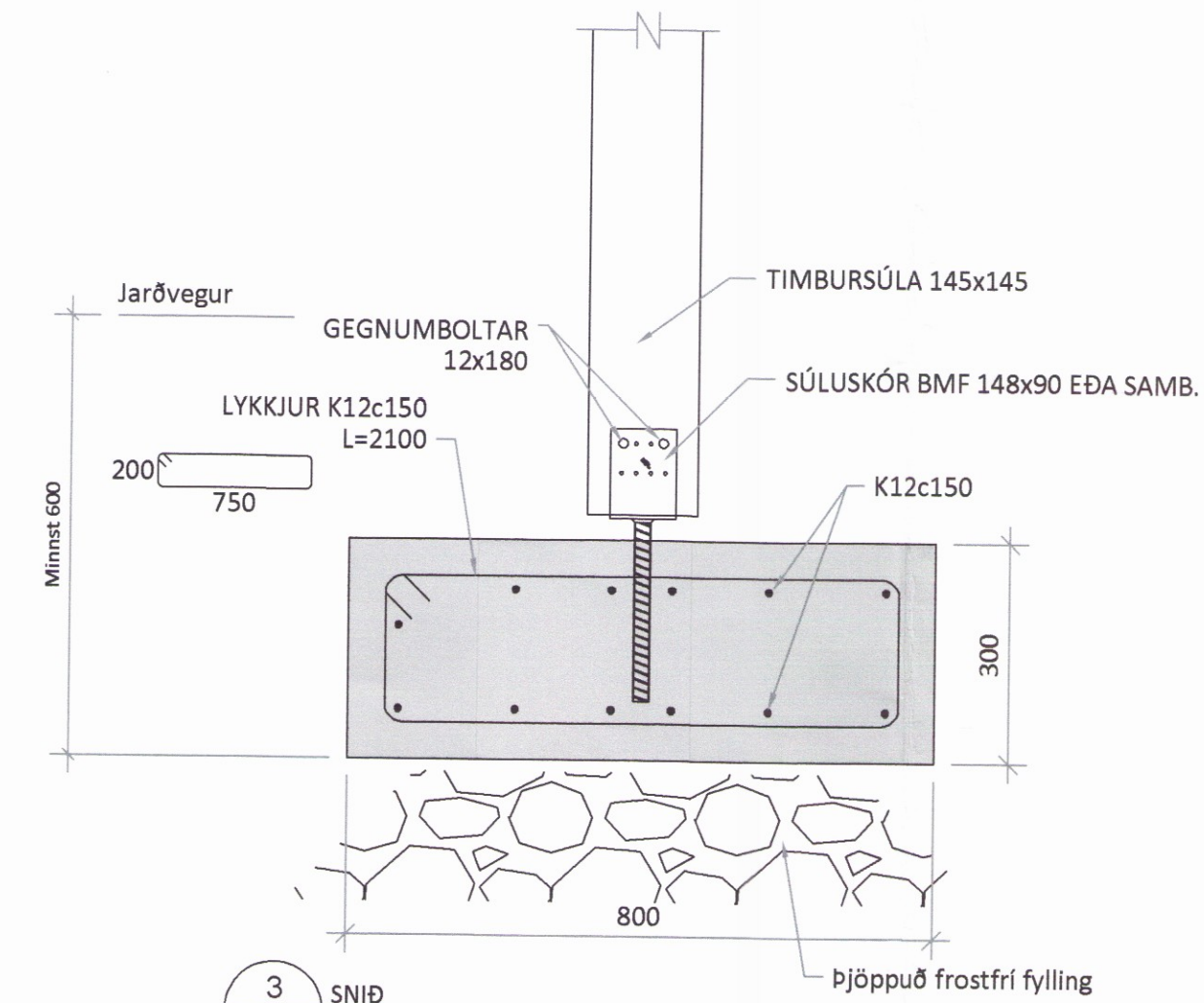
3 SNID 101 | 102 Mkv. 1:10
