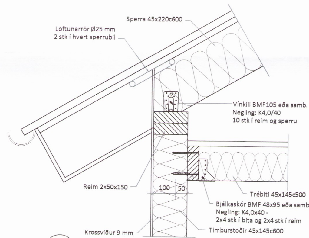
5 SNID 101 | 102 Mkv. 1:10
