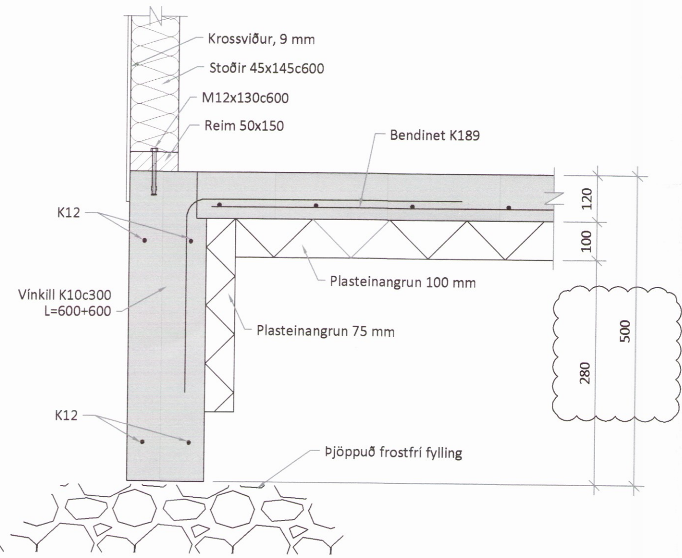
1 SNID 101 | 102 Mkv. 1:10
