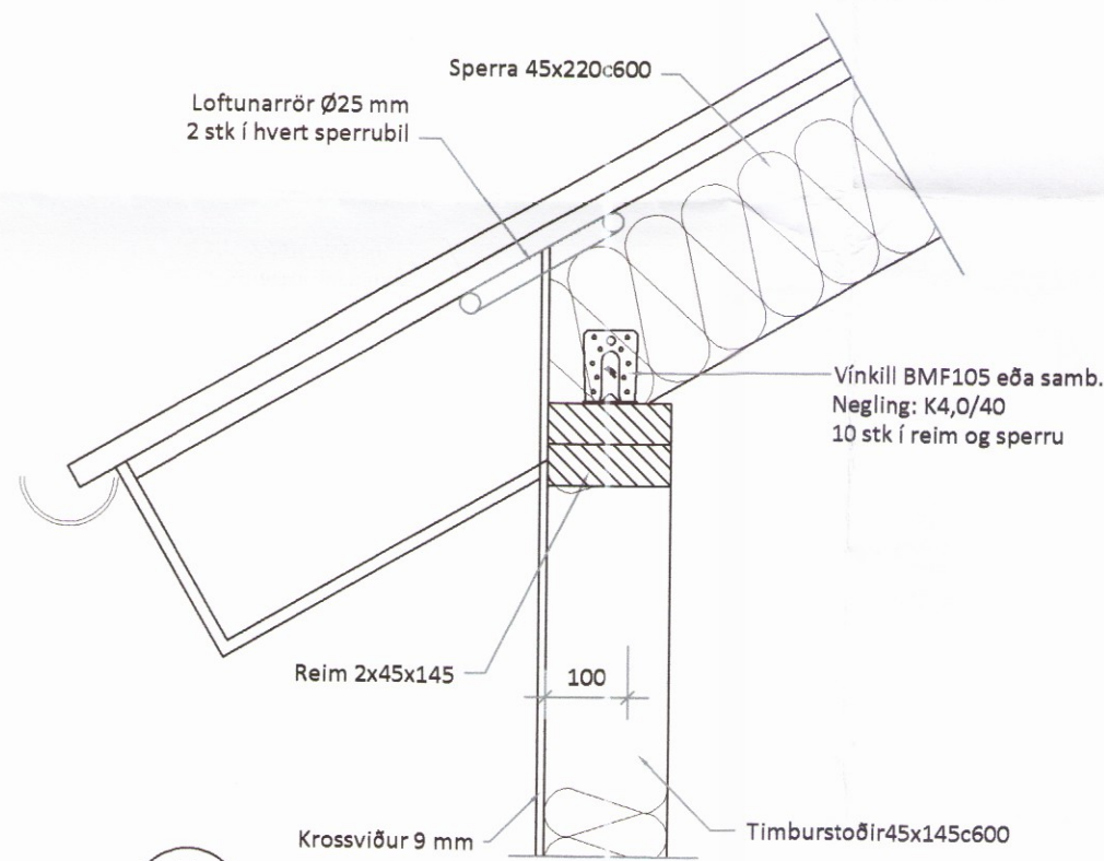
6 SNID 101 | 102 Mkv. 1:10
