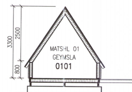
SNID 3-3 1:100
