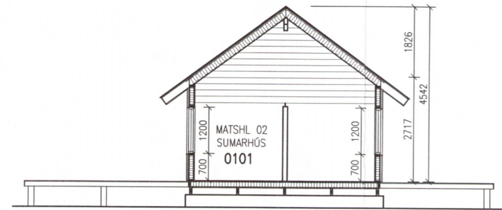
SNID 2-2 1:100
