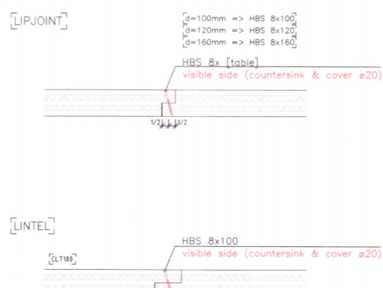
D03 connection: Lipjoint standard Lipjoint and Lintel
