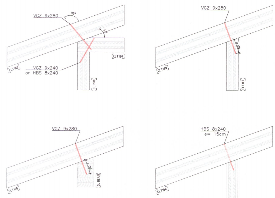
D06 connection: roof standard - wall-ceiling-roof - wall-roof - beam-roof
