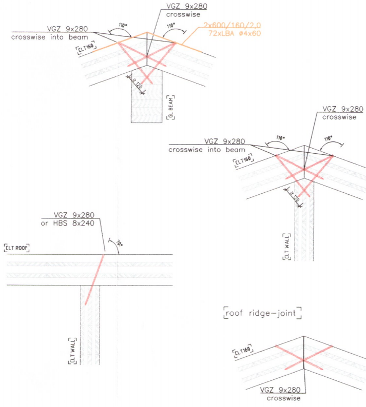
D10 connection: roof top standard glulam + wall
