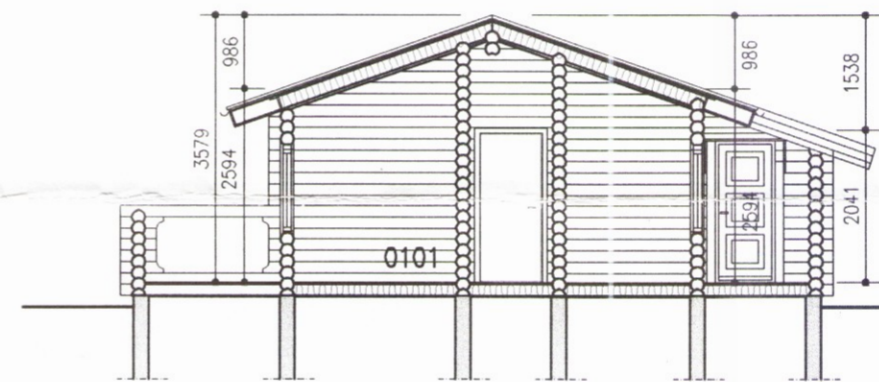
SNID 2-2 1:100
