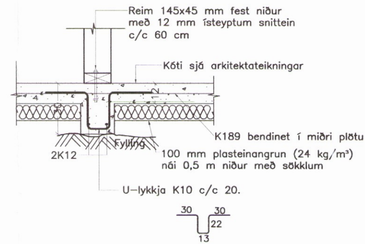
C SNID C-C. 1:20.
