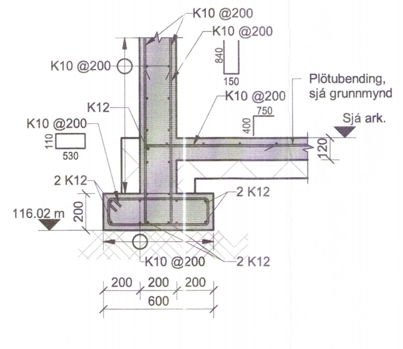
AS Snið AS 00_1_21_01 1 : 20
