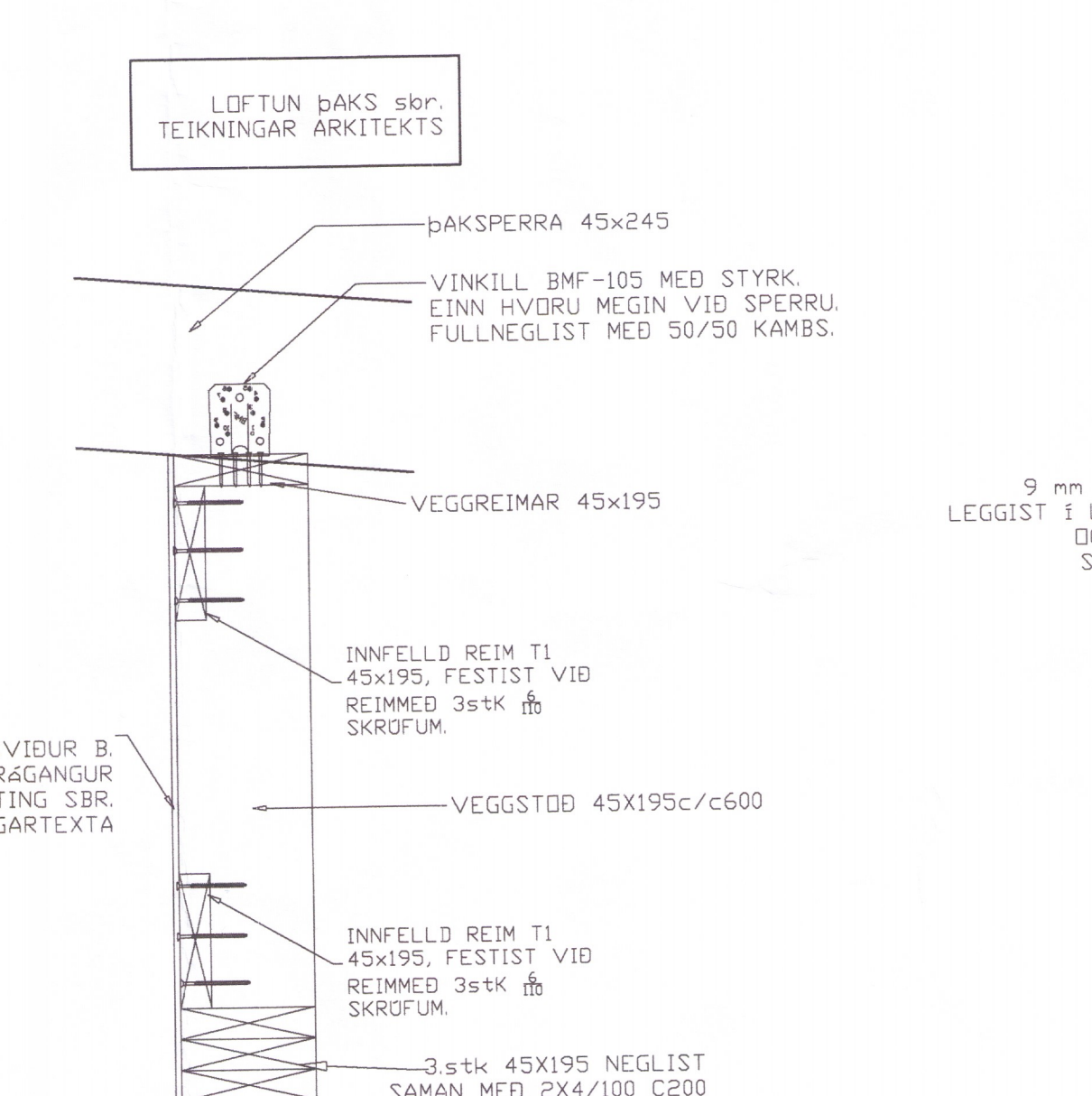
FESTING, F7 1:10
