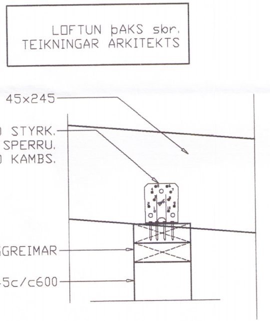
FESTING, F4 1:10
