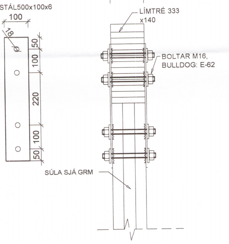
FESTING, F3 1:10
