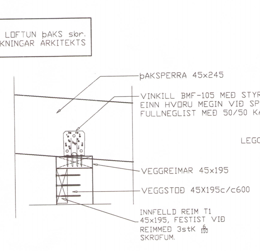
FESTING, F6 1:10
