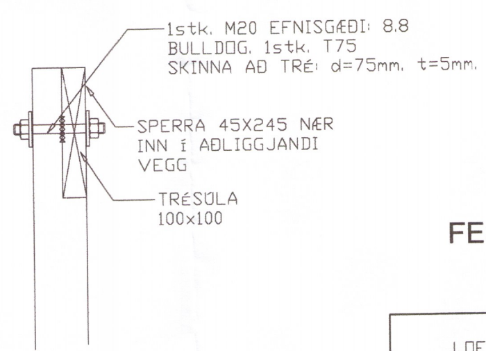
FESTING, F5 1:10
