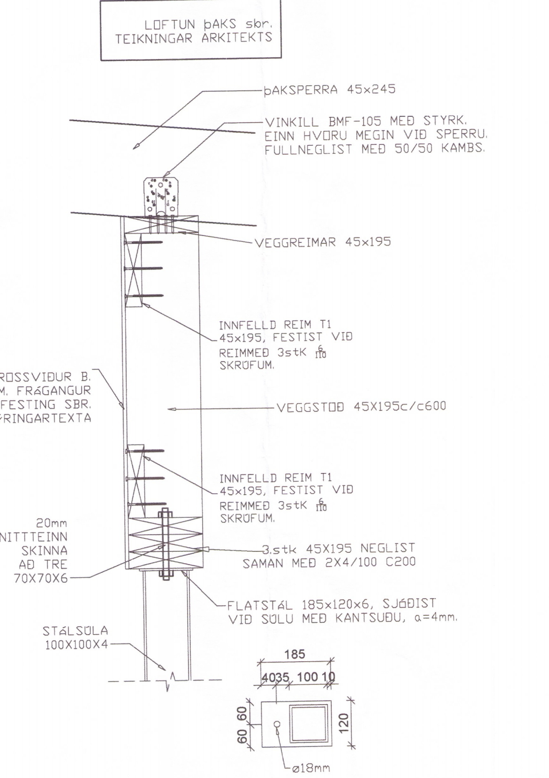
FESTING, F9 1:10
