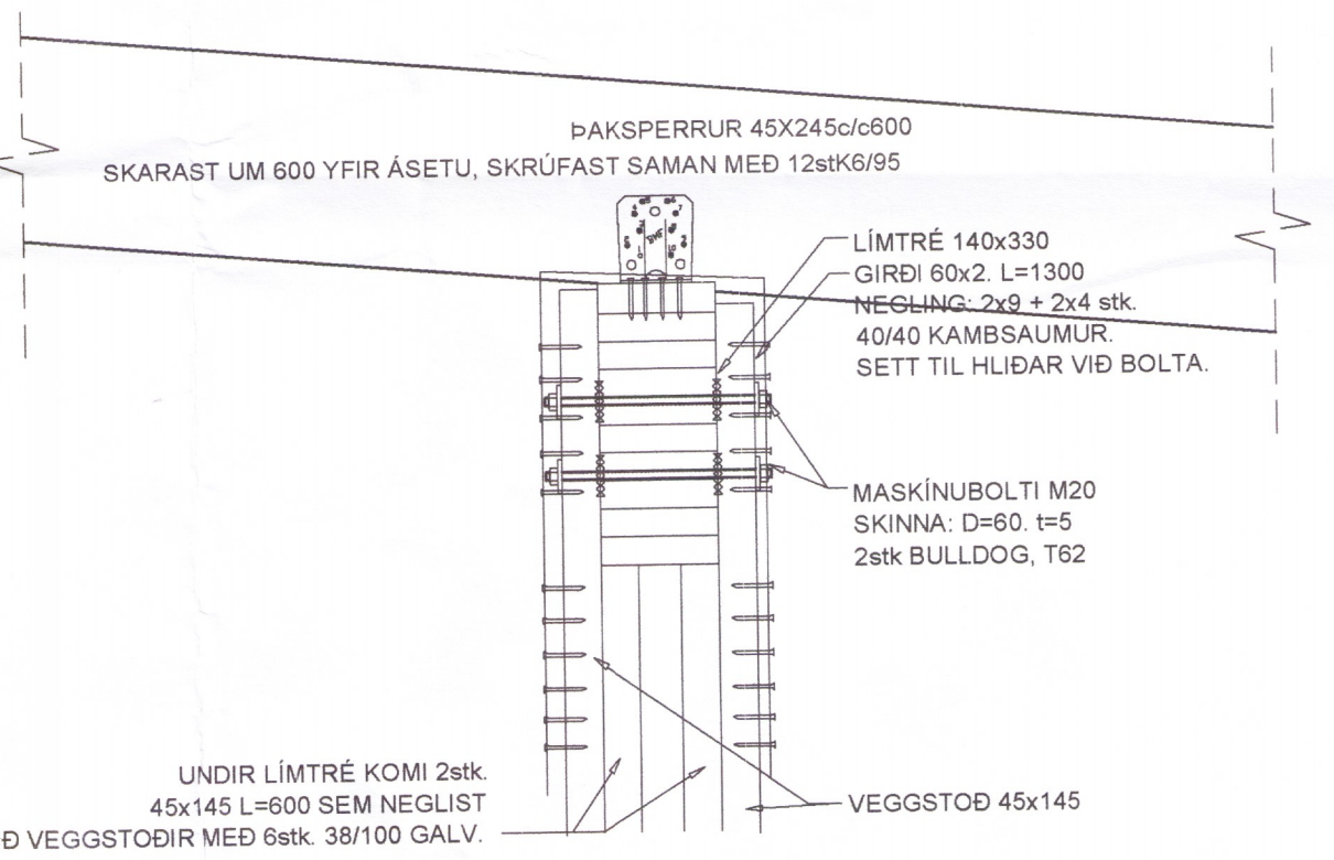
FESTING, F4 1:10
