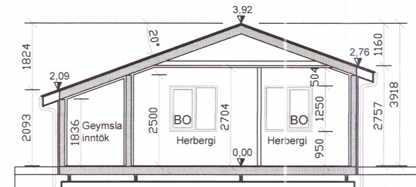
SNID A - 1:100
