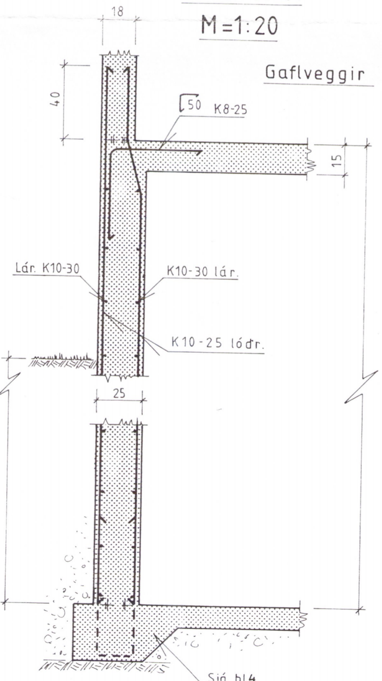
Snid V4-V4 M=1:20
