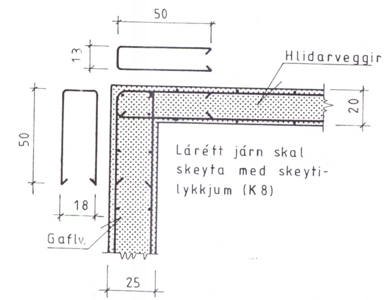
Horn M=1:20 (Lárétt snid)
