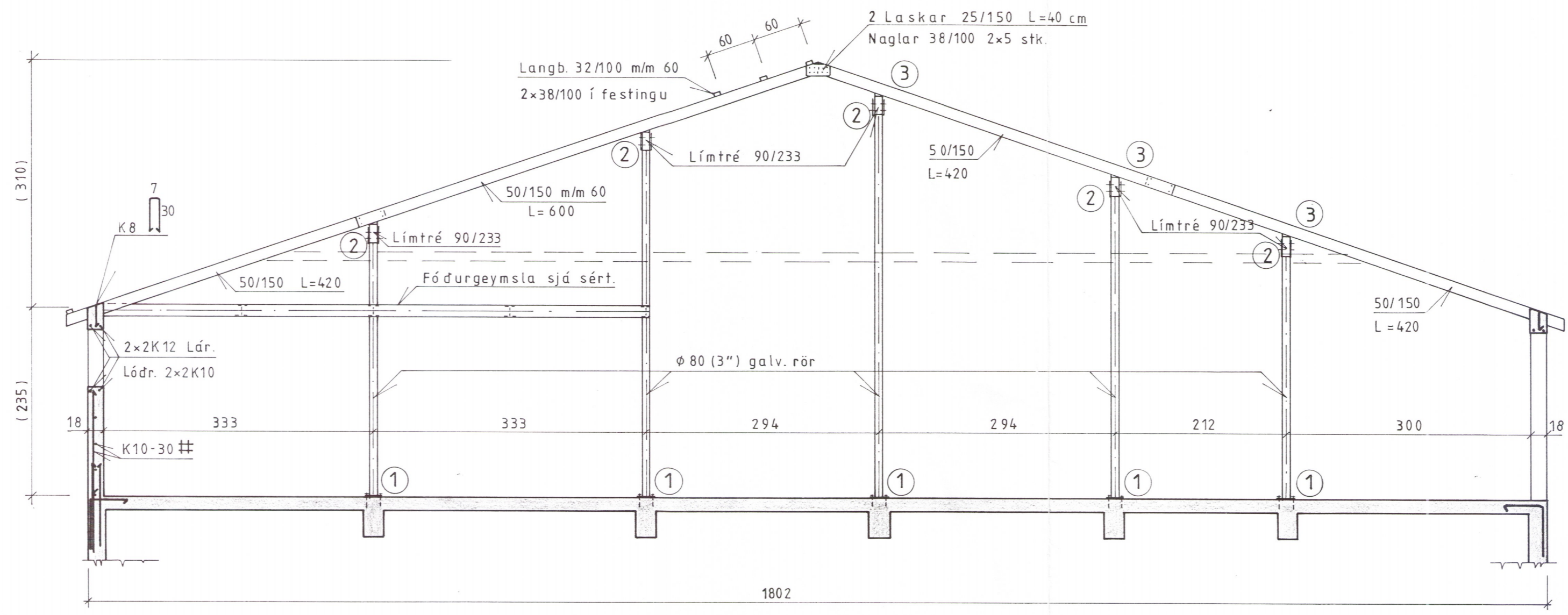
Snid p-p M=1:50
