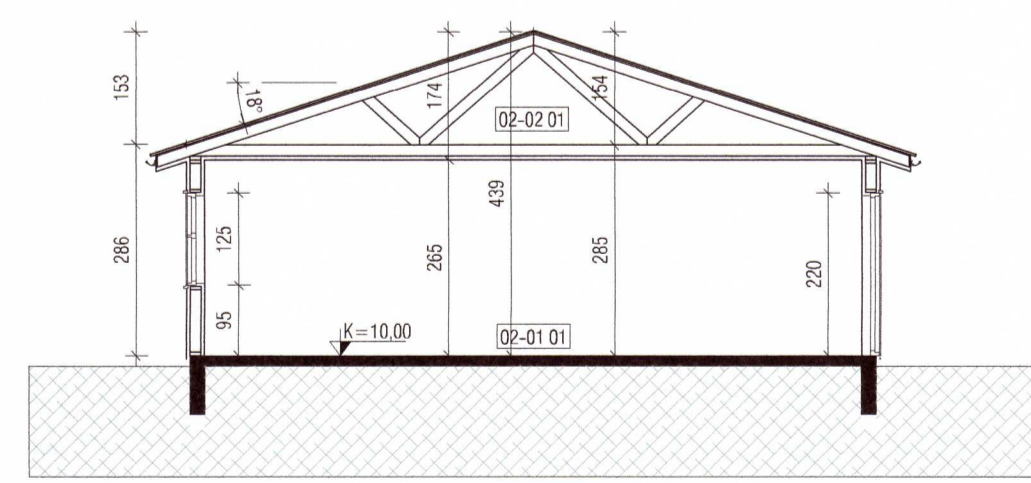
SNID C-C 1:100
