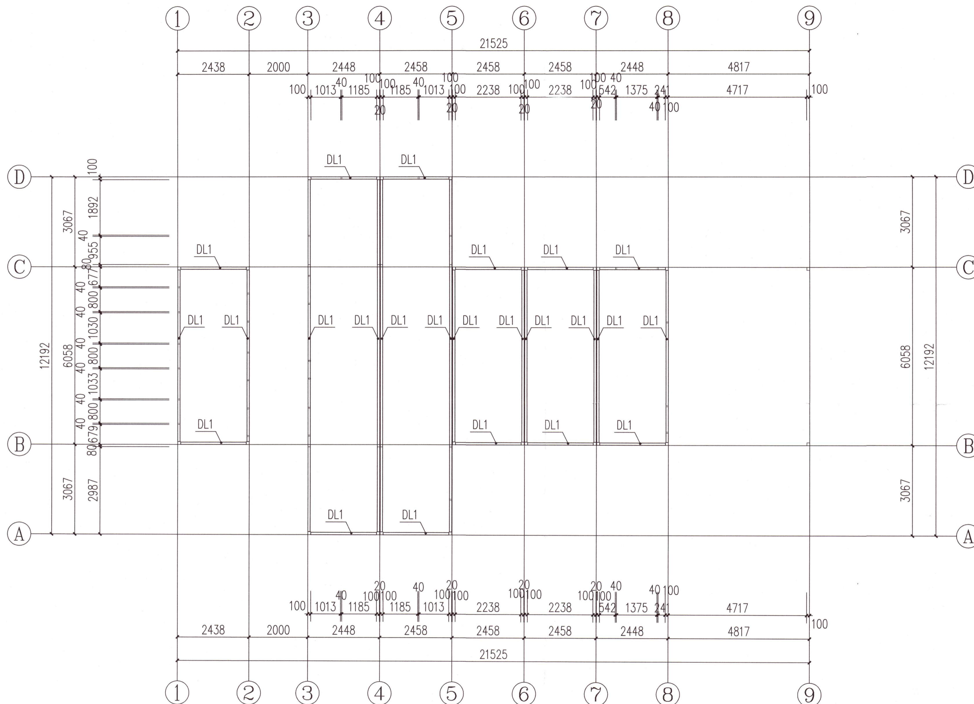
Floor beam Layout 1:100
