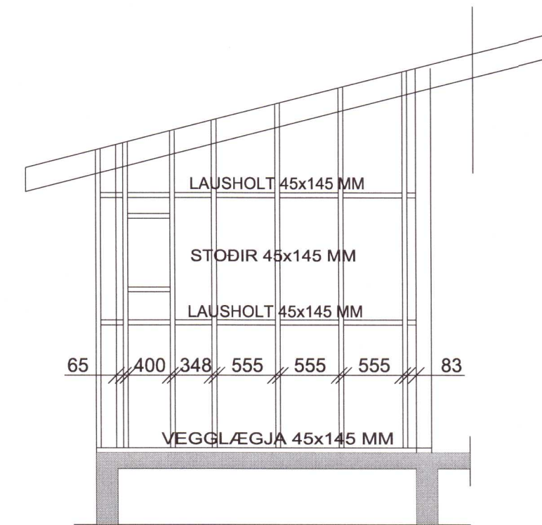
SNID - F 1:50
