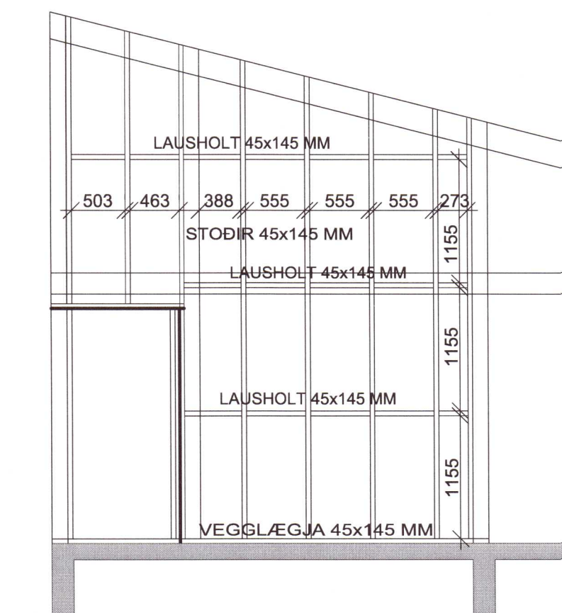
SNID - H 1:50
