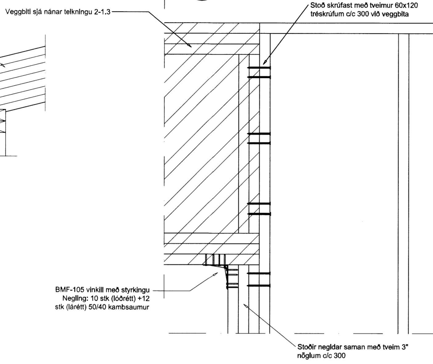
F7 Festing F7 2-1.1 1:10
