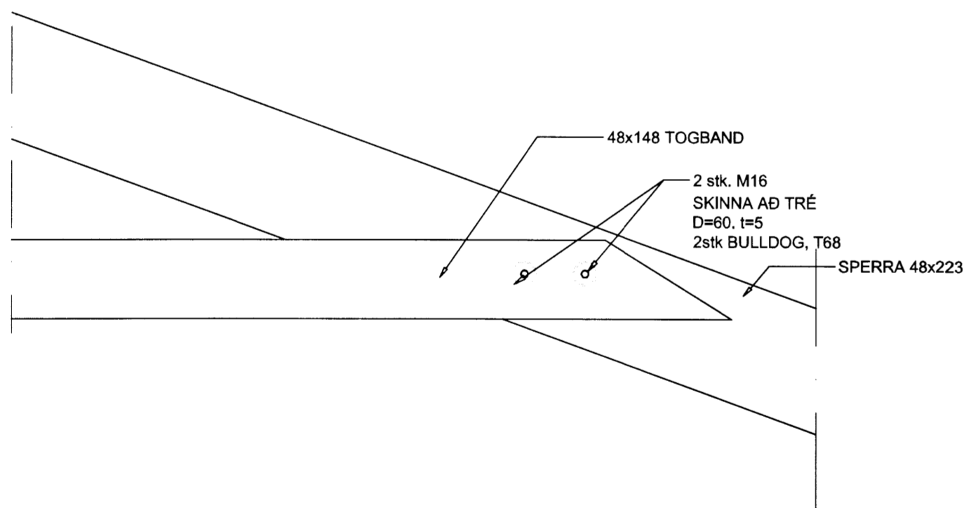
FESTING F3 1:10
