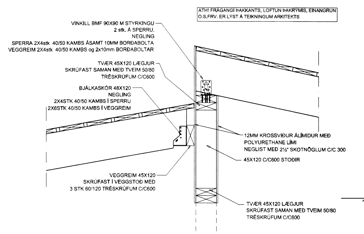
FESTING F4 1:10
