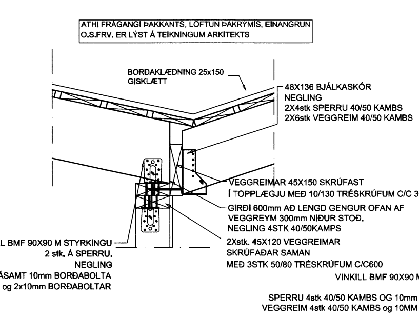
Festing F3 1:10
