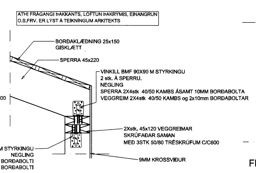
FESTING F5 1:10
