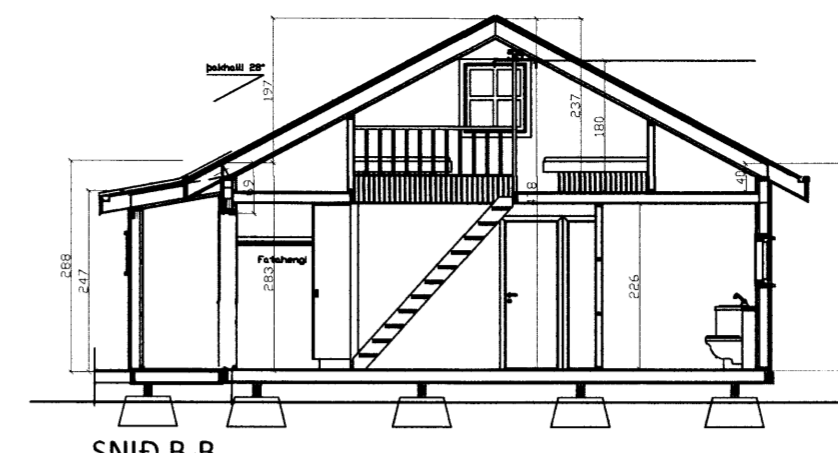
SNID B-B
