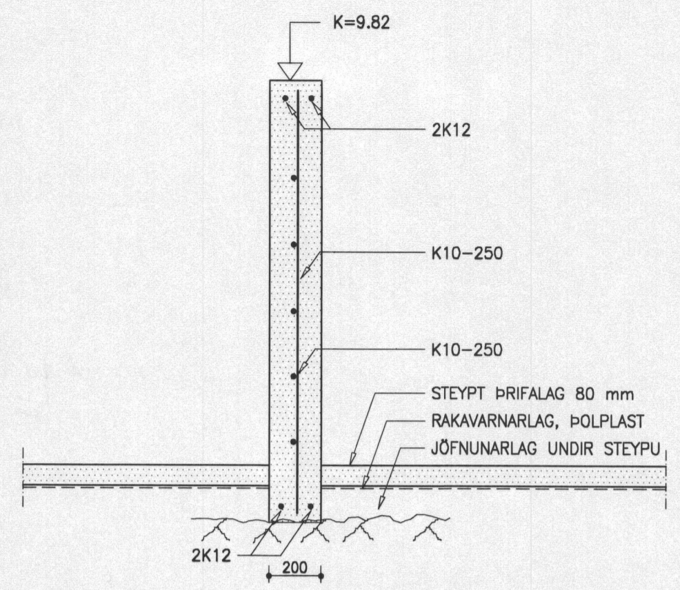
SNID 2-2 1:20
