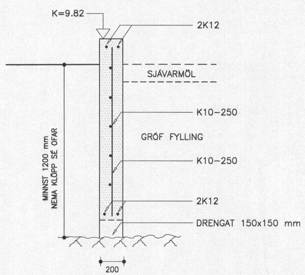
SNID 3-3 1:20
