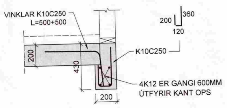
H SNEIÐING 03 Mkv. 1/20
