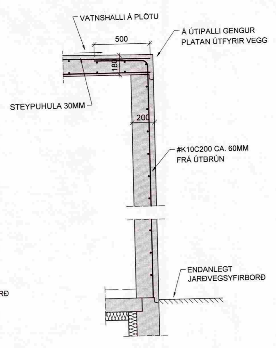
F SNEIÐING 03 Mkv. 1/20
