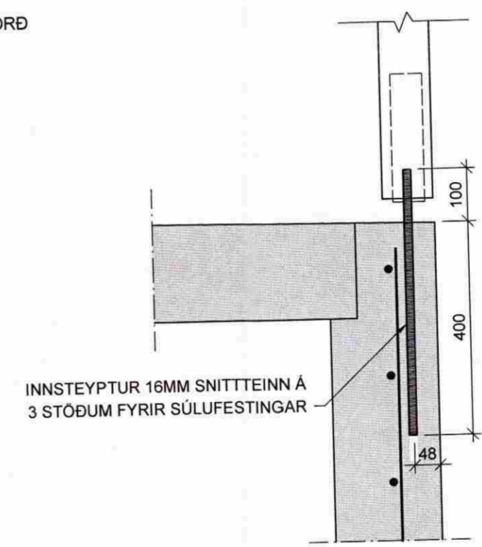
X SNEIÐING 03 Mkv. 1/20
