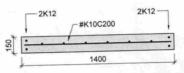
V1 VEGGUR 03 Mkv. 1/20
