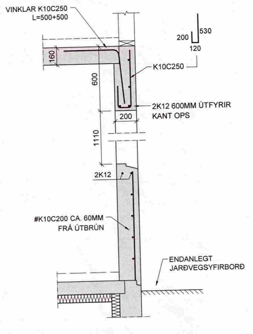
G SNEIÐING 03 Mkv. 1/20
