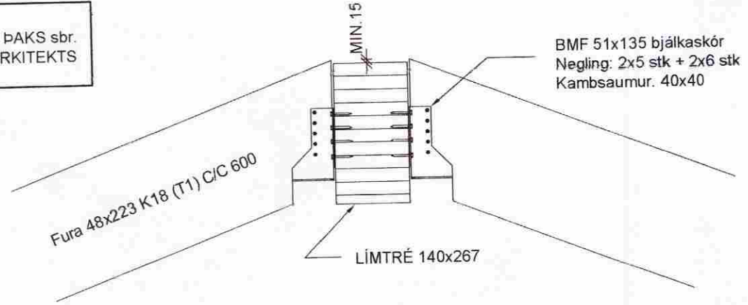
FESTING, F 2:10
