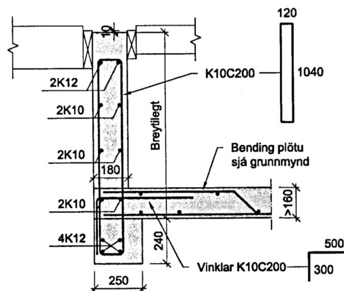
N SNEIÐING 03 Mkv. 1/20
