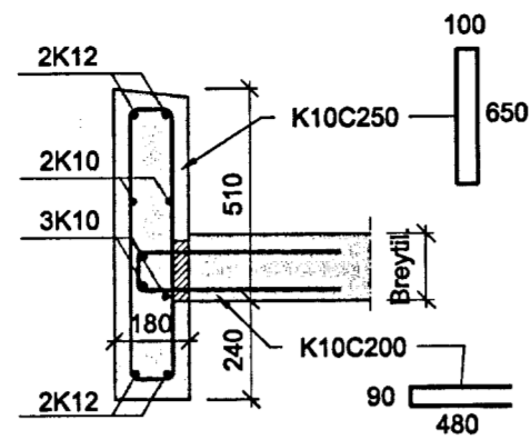
J SNEIÐING 03 Mkv. 1/20
