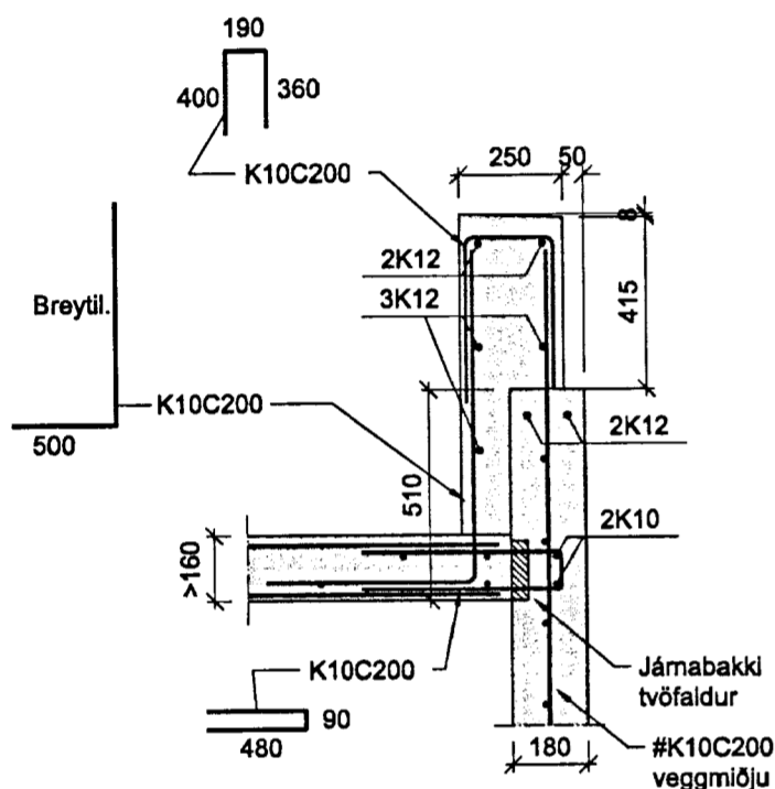
M SNEIÐING 03 Mkv. 1/20
