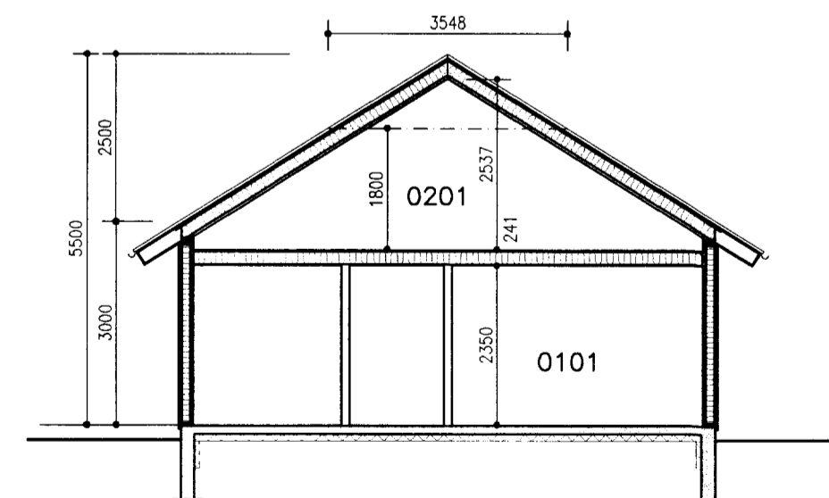
SNID 2-2 1:100
