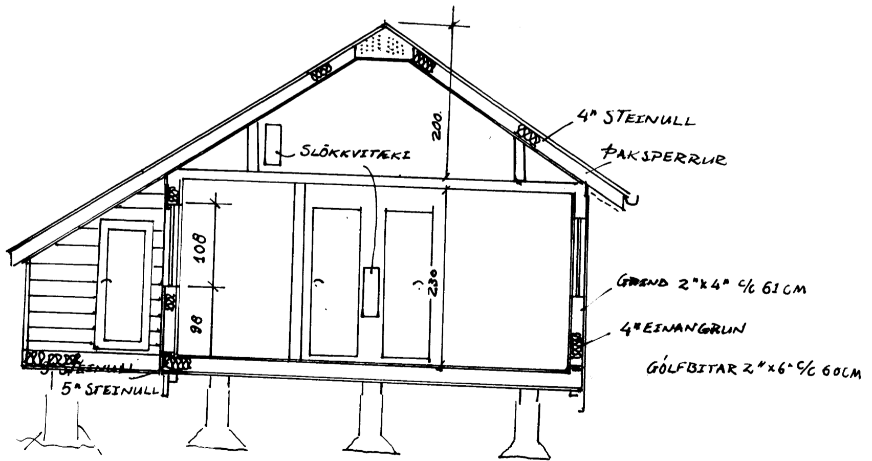
SNED A-A
