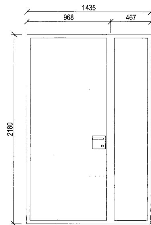
H-01, 1.stk M= 1:25
