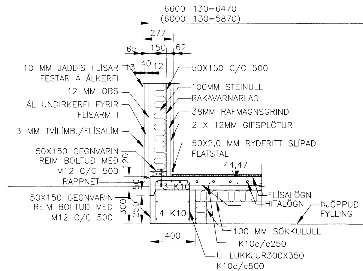
SNID 1:20
