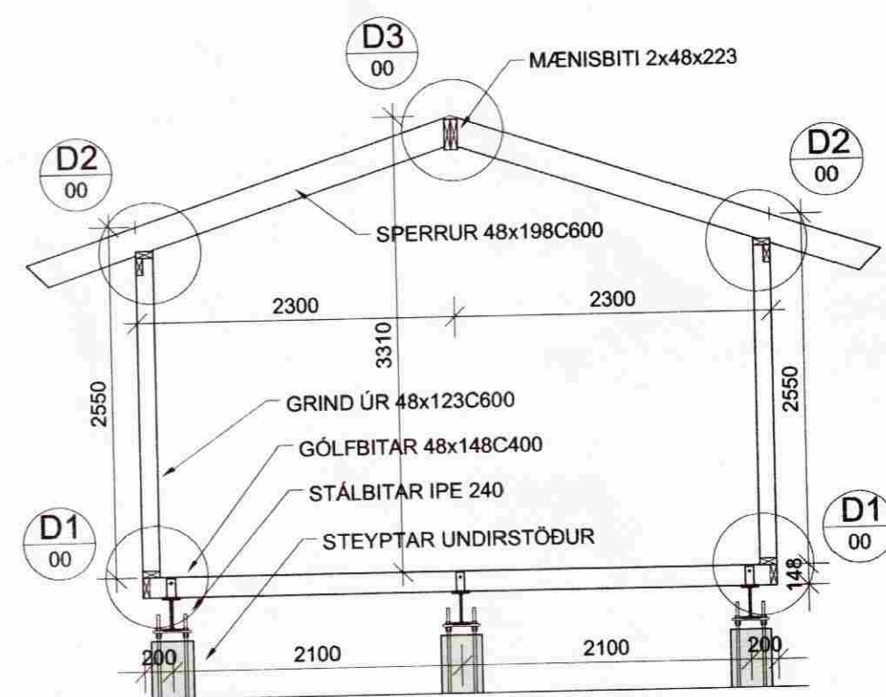
A SNEIÐING 00 Mkv. 1/50
