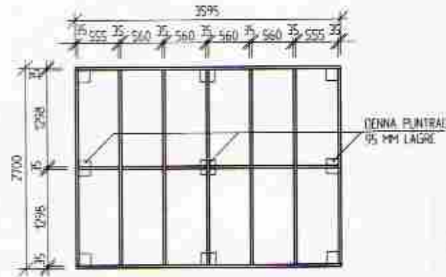
BOTTENBJÄLKLAG FLOOR STRUCTURE LEVEL
