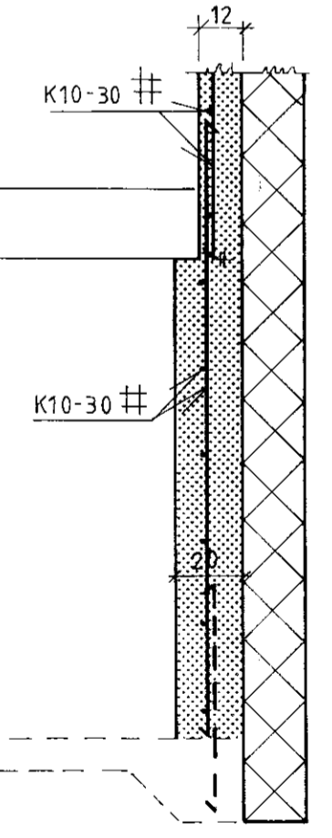
Snid 3-3 M=1:20
