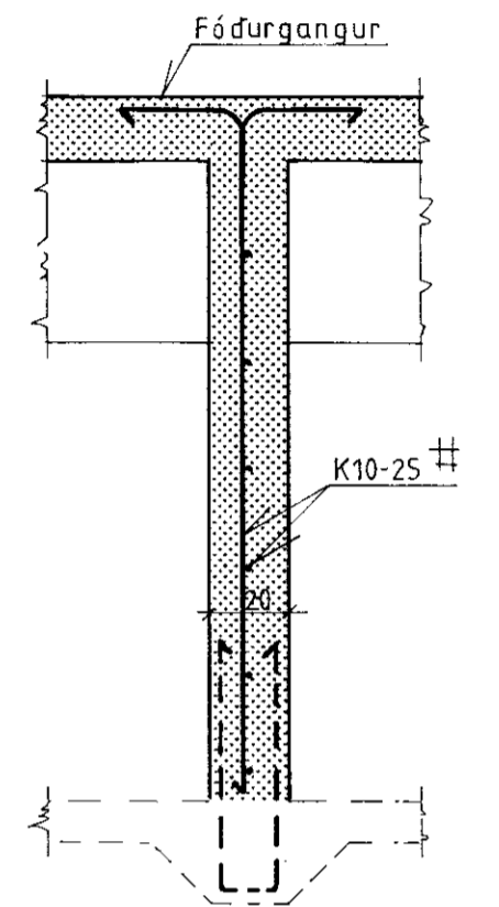
Snid 4-4 M=1:20
