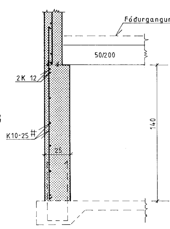
Snid 1-1 M=1:20
