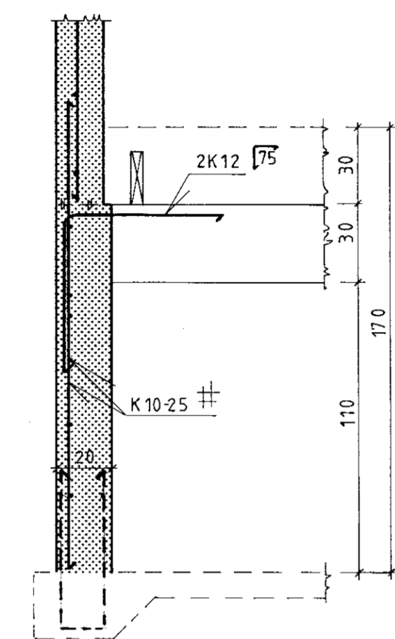
Snid 2-2 M=1:20
