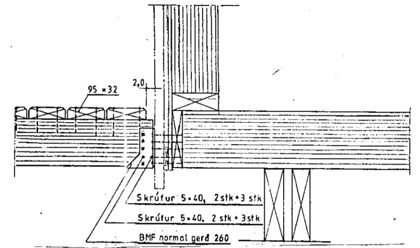
Snid E-E
