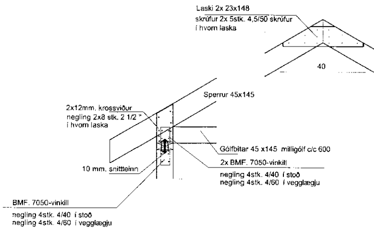
SNID C-C 1:20
