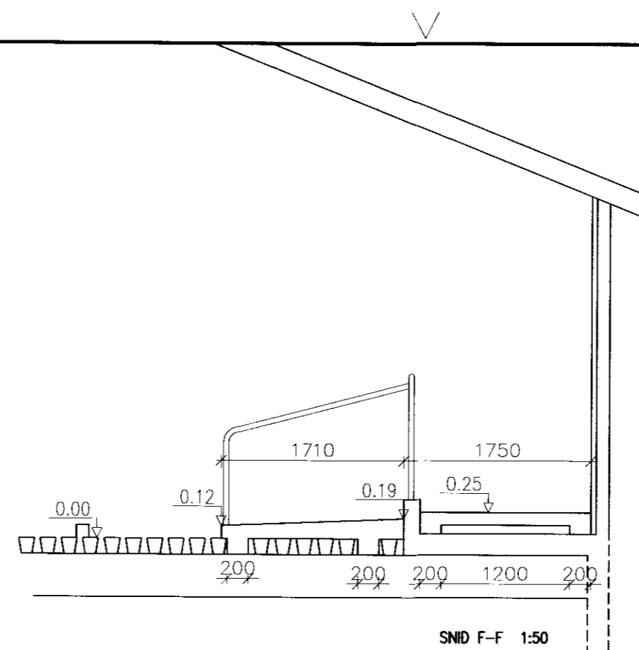
SNID F-F 1:50
